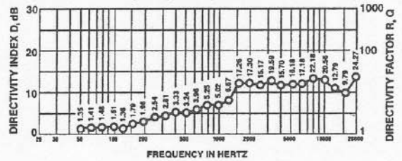
FIGURE 6 — Sx200a Directivity Response (anechoic environment)
